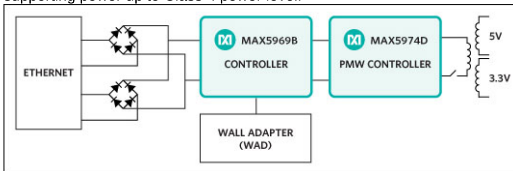
Figure 1. The Pasadena subsystem design block diagram.
